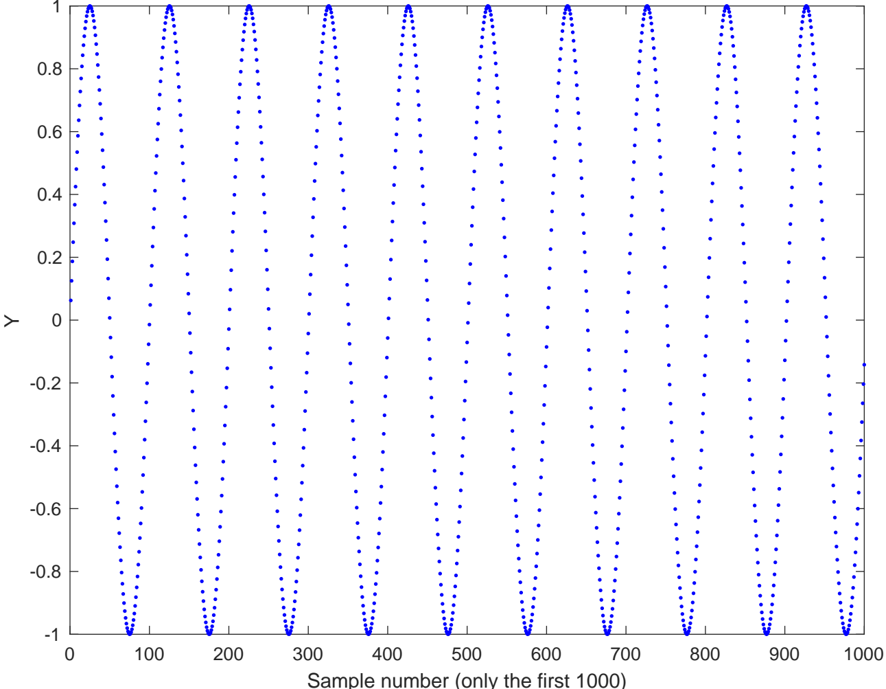
The wave for a 440 Hz sine, sampled at 44,100 Hz
