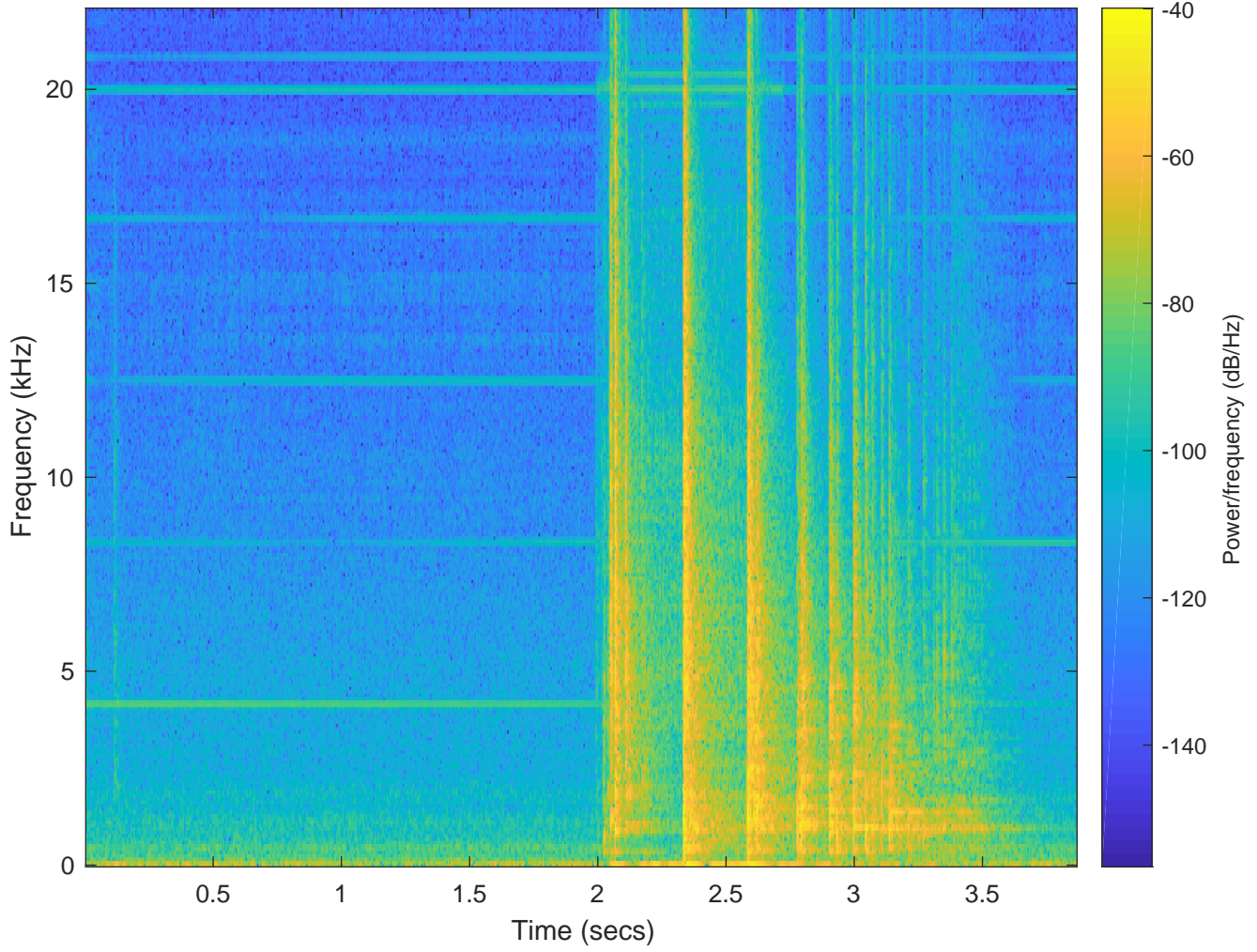
Spectrogram for the sound generated by a robot dropping a pop can
