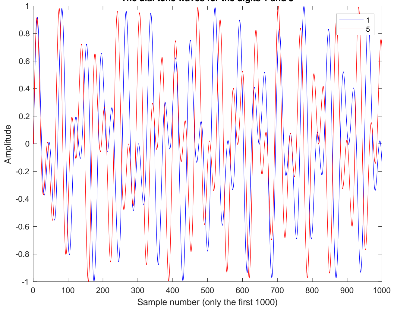
The dial tone waves for the digits 1 and 5
