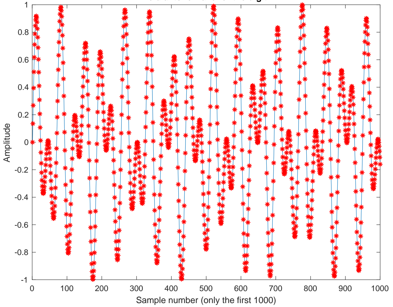
The dial tone wave for the digit 1
