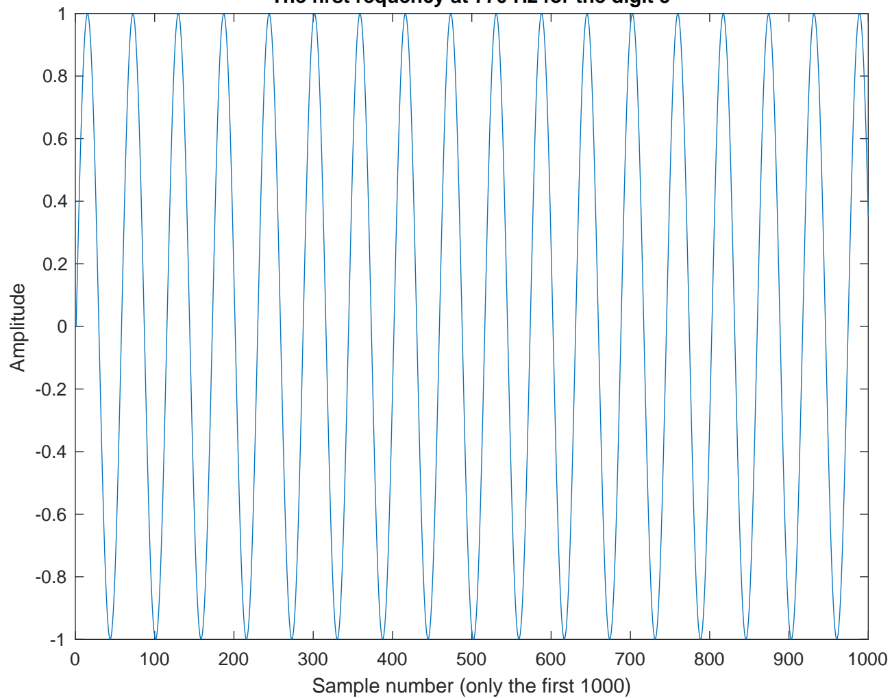
The first frequency at 770 Hz for the digit 5
