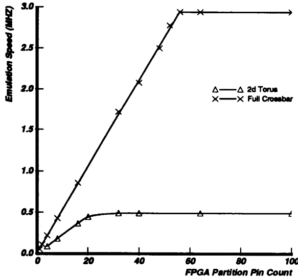
Figure 11: A-1000 Emulation Speed (Communication only Component)
