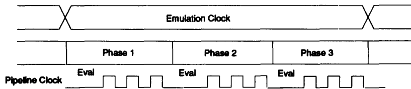
Figure 4: Emulation Phase Clocking Scheme
