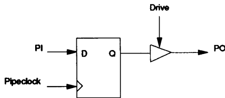
Figure 8: Intermediate Hop Pipeline Stage
