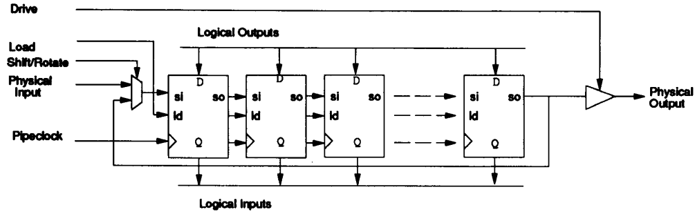
Figure 6: Shift Loop Architecture
