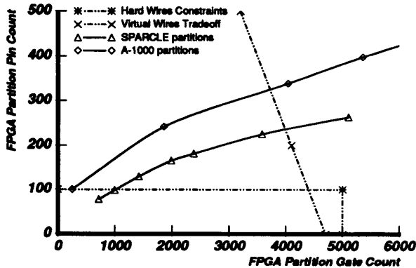
Figure 10: Determination of optimal partition size
