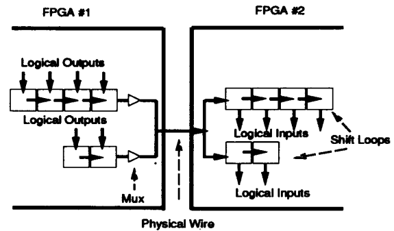
Figure 3: Virtual Wire Interconnect
