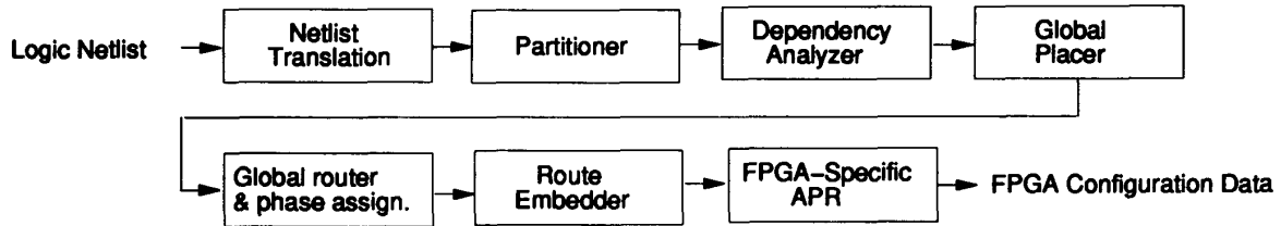
Figure 5: Software Tool Flowchart
