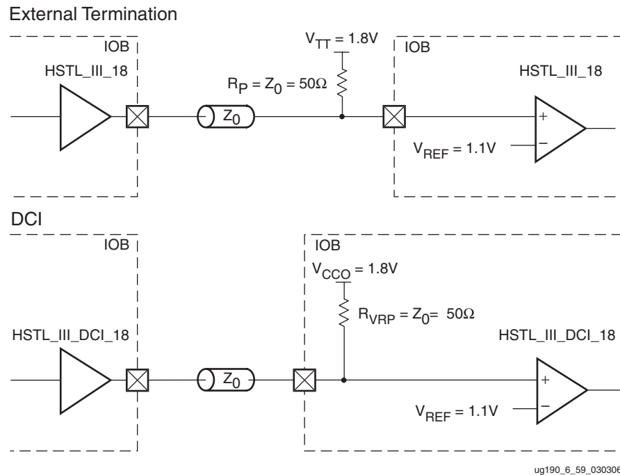
Figure 6-60: HSTL Class III (1.8V) Termination
