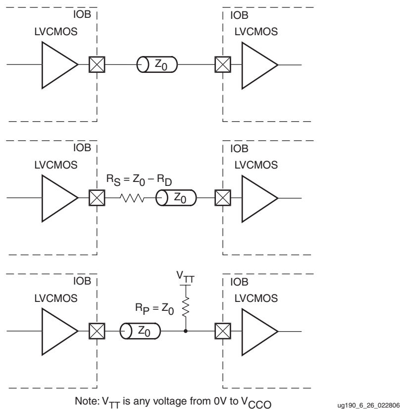
Figure 6-26: LVCMOS Unidirectional Termination
