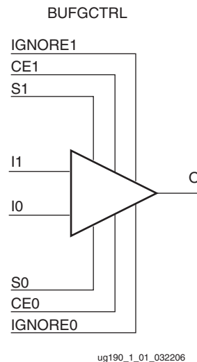
Figure 1-1: BUFGCTRL Primitive
