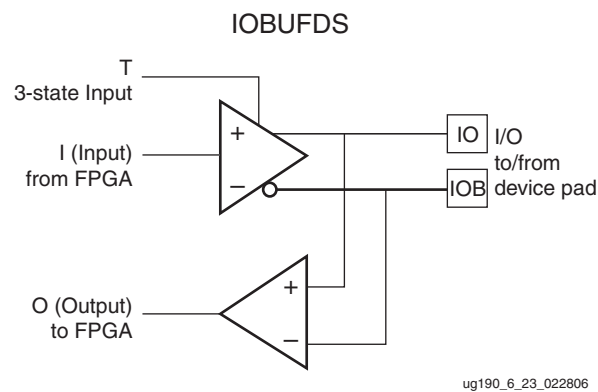
Figure 6-23: Differential Input/Output Buffer Primitive (IOBUFDS)
