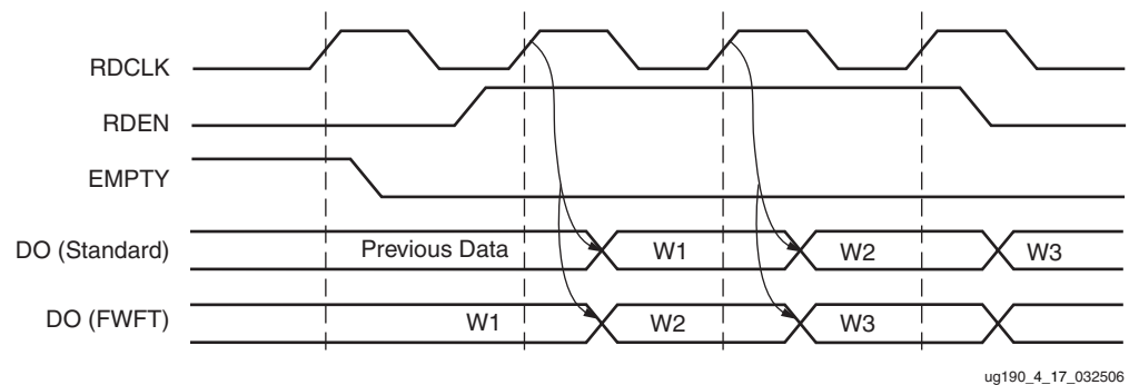
Figure 4-19: Read Cycle Timing (Standard and FWFT Modes)
