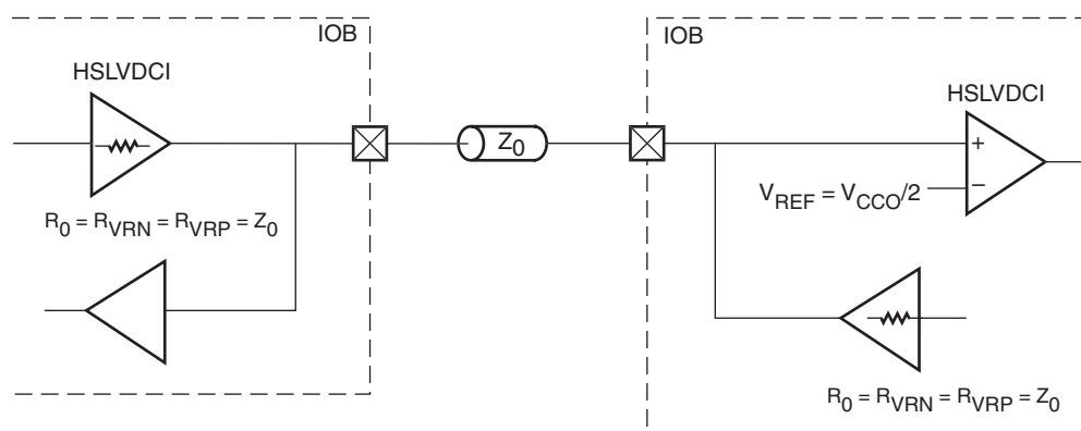
Figure 6-33: HSLVDCI Controlled Impedance Driver with Bidirectional Termination
