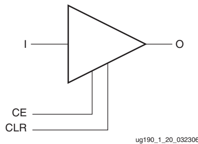
Figure 1-20: BUFR Primitive
