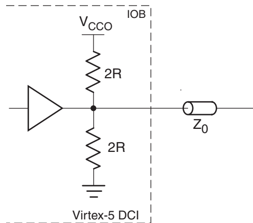
Figure 6-13: Driver with Termination to V_{CCO}/2 Using DCI Split Termination
