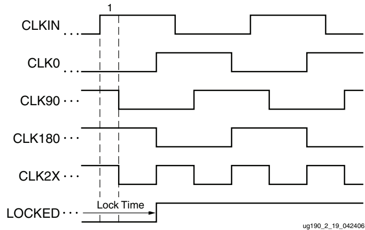
Figure 2-19: Phase Shift Example: Fixed
