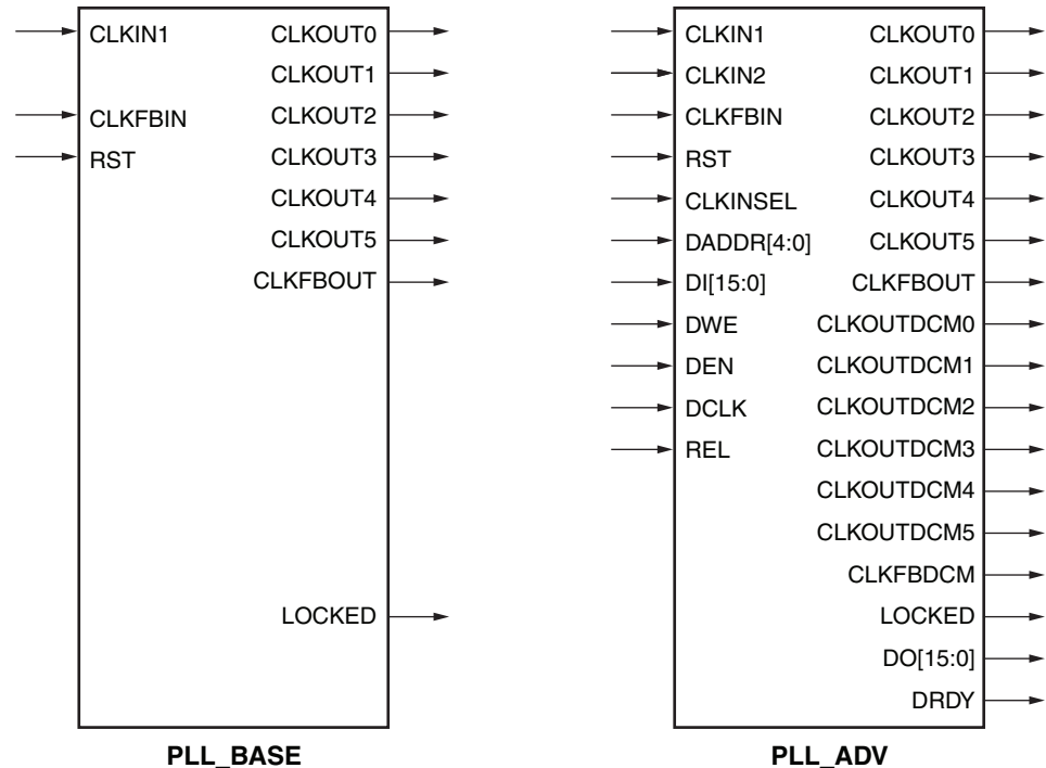
Figure 3-4: PLL Primitives
