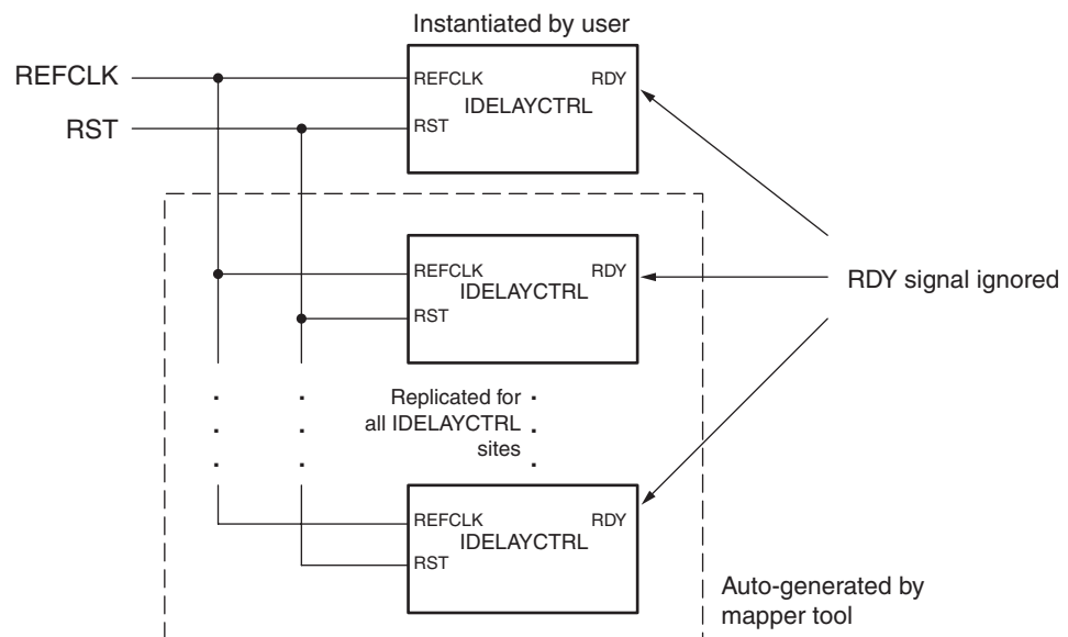
Figure 7-13: Instantiate IDELAYCTRL Without LOC Constraints - RDY Unconnected
