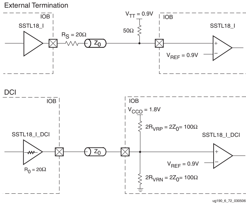
Figure 6-75: SSTL18 (1.8V) Class I Termination
