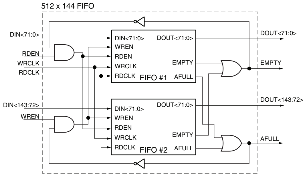
Figure 4-26: Cascading FIFO by Width
