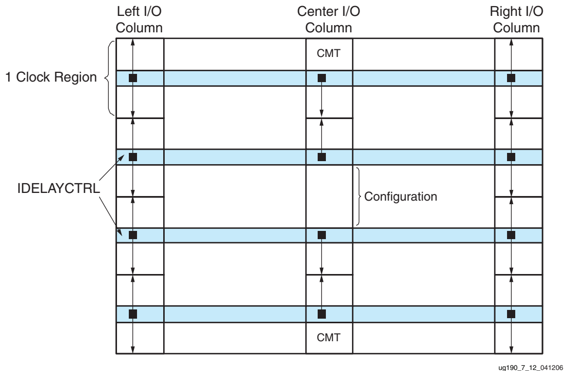
Figure 7-12: Relative Locations of IDELAYCTRL Modules
