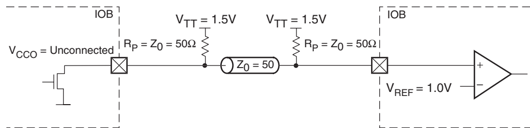
Figure 6-36: GTL+ with External Parallel Termination and Unconnected V_{CCO}
