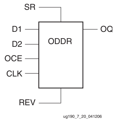
Figure 7-20: ODDR Primitive Block Diagram
