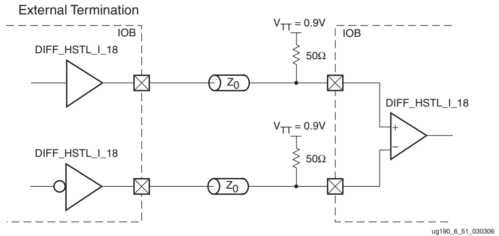
Figure 6-52: Differential HSTL (1.8V) Class I Unidirectional Termination
