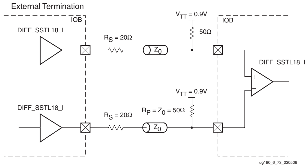
Figure 6-76: Differential SSTL (1.8V) Class I Unidirectional Termination
