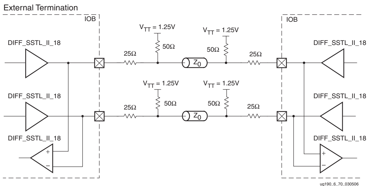
Figure 6-72: Differential SSTL2 (2.5V) Class II with Bidirectional Termination
