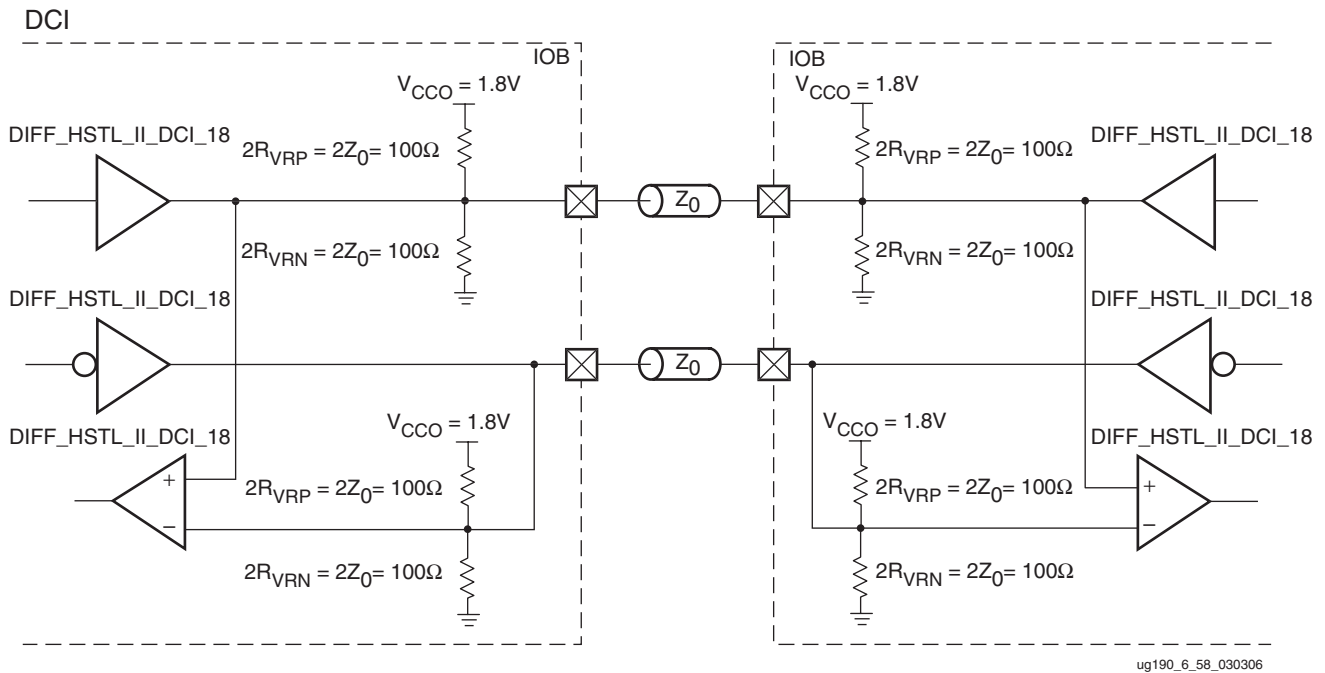
Figure 6-59: Differential HSTL (1.8V) Class II DCI Bidirectional Termination
