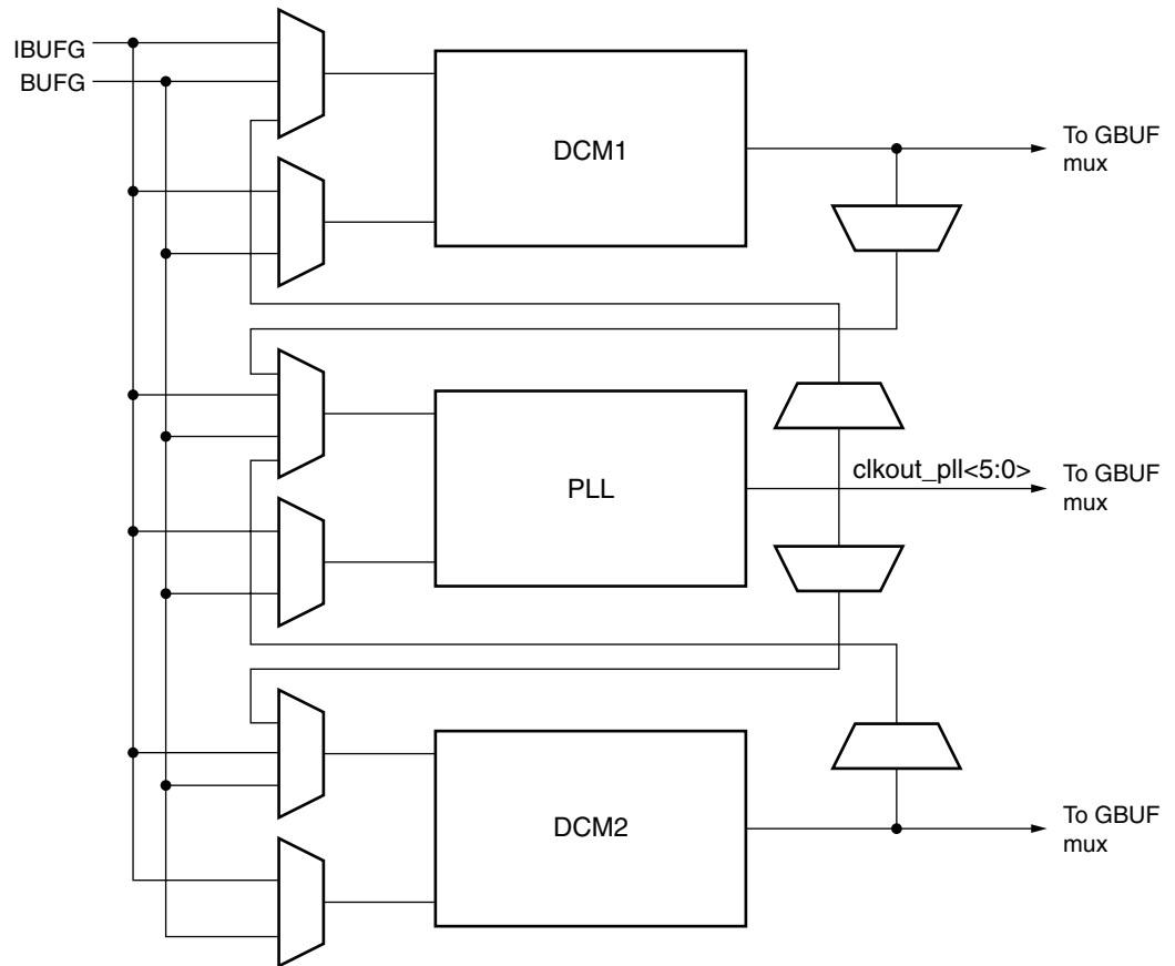
Figure 3-1: Block Diagram of the Virtex-5 CMT
