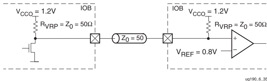
Figure 6-35: GTL_DCI with Internal Parallel Driver and Receiver Termination
