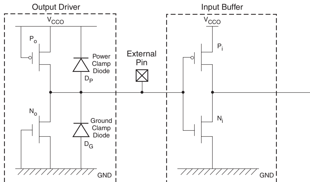
Figure 6-89: Virtex-5 I/O: 3-State Output Driver
