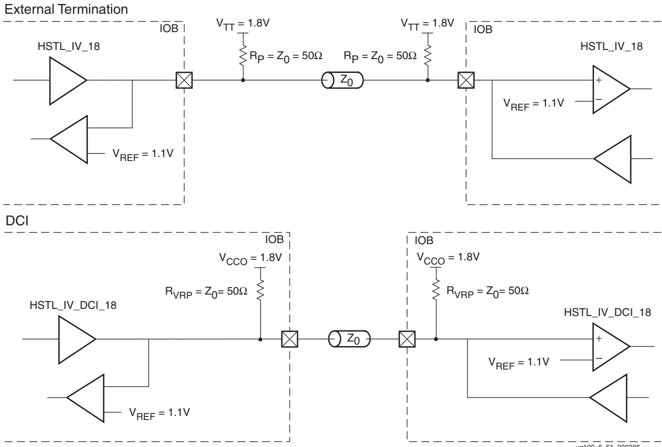
Figure 6-62: HSTL Class IV (1.8V) with Bidirectional Termination
