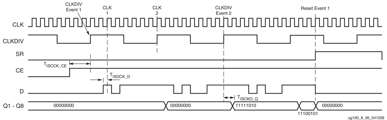
Figure 8-6: 8:1 SDR ISERDES
