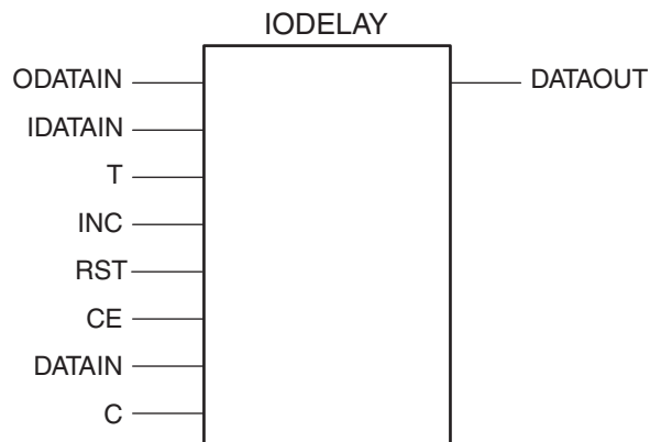
Figure 7-8: IODELAY Primitive
