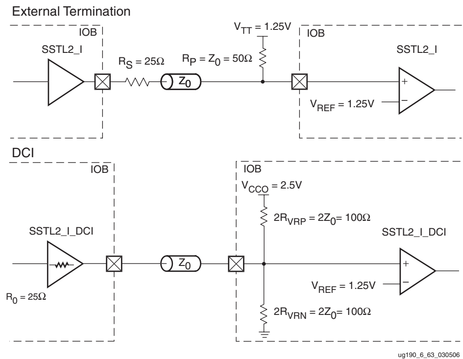
Figure 6-65: SSTL2 Class I Termination
