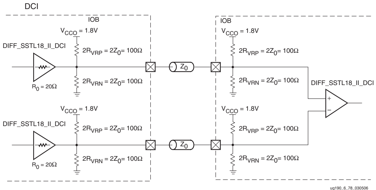
Figure 6-81: Differential SSTL (1.8V) Class II Unidirectional DCI Termination
