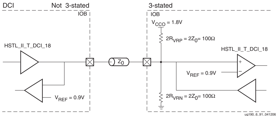
Figure 6-63: HSTL_II_T_DCI_18 Split-Thevenin Termination
