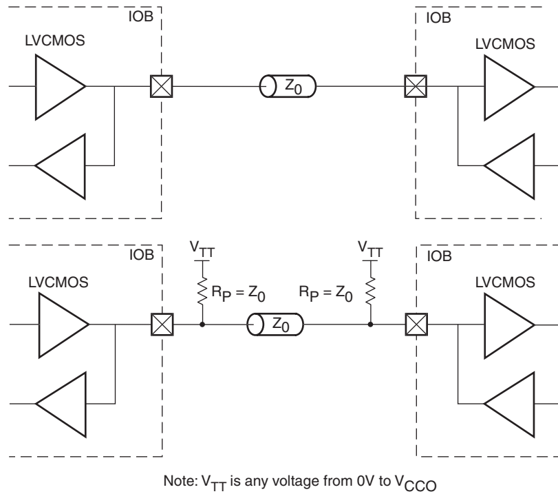
Figure 6-27: LVC MOS Bidirectional Termination
