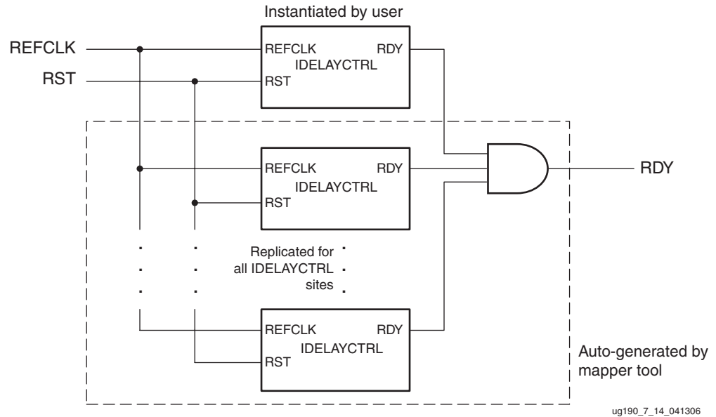
Figure 7-14: Instantiate IDELAYCTRL Without LOC Constraints - RDY Connected
