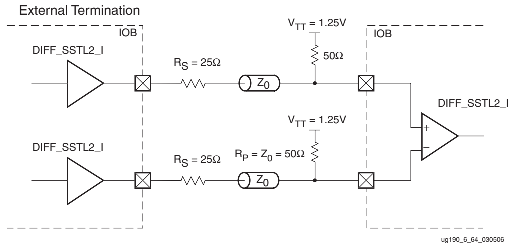
Figure 6-66: Differential SSTL2 Class I Unidirectional Termination
