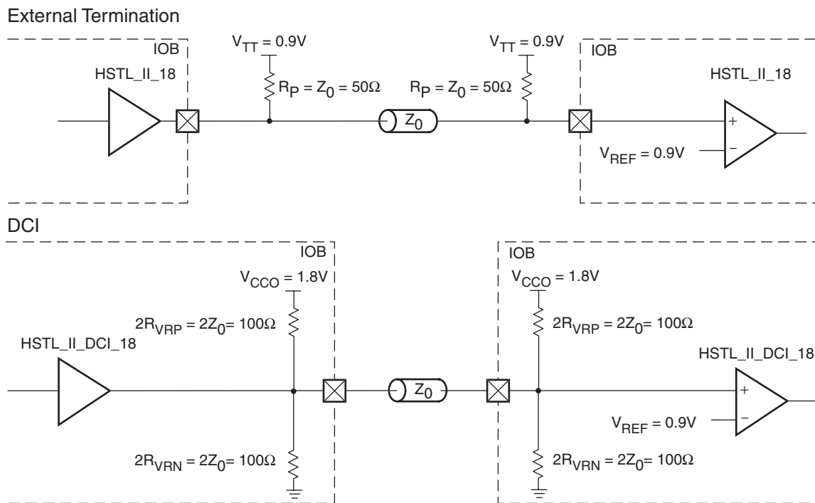
Figure 6-54: HSTL Class II (1.8V) with Unidirectional Termination
